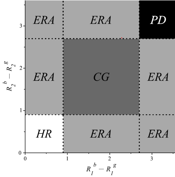
Figure 2: Various types of games arising for different parametrizations
