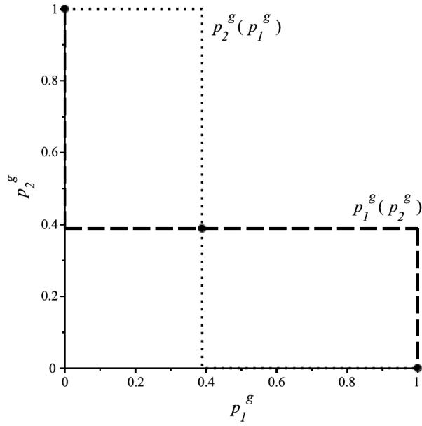
Figure 1: Best-response functions in a Chicken Game
